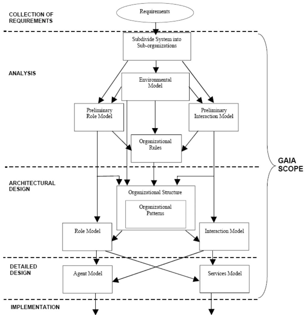
Figura 20 - Models of the Gaia methodology and their relations in the Gaia process (Zambonelli, Jennings, & Wooldrige).
