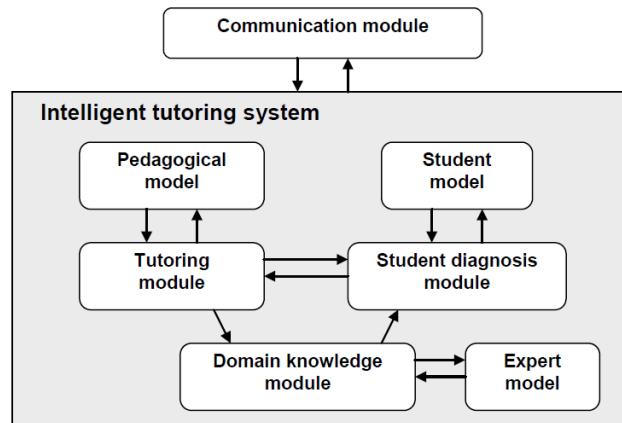
Figura 17 - Core architecture of intelligent tutoring system(Grundspenkis, 2011)
