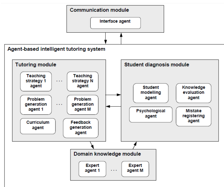
Figura 18 - Architecture of agent-based ITS (Grundspenkis, 2011)
